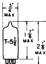
GLASS BULB MINIATURE BUTTON 7 PIN BASE E7-1 OUTLINE DRAWING JEDEC 9-2
